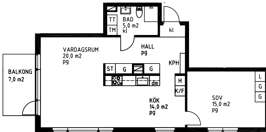
PLAN 3
