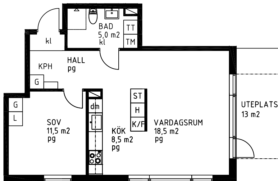
PLAN 1
