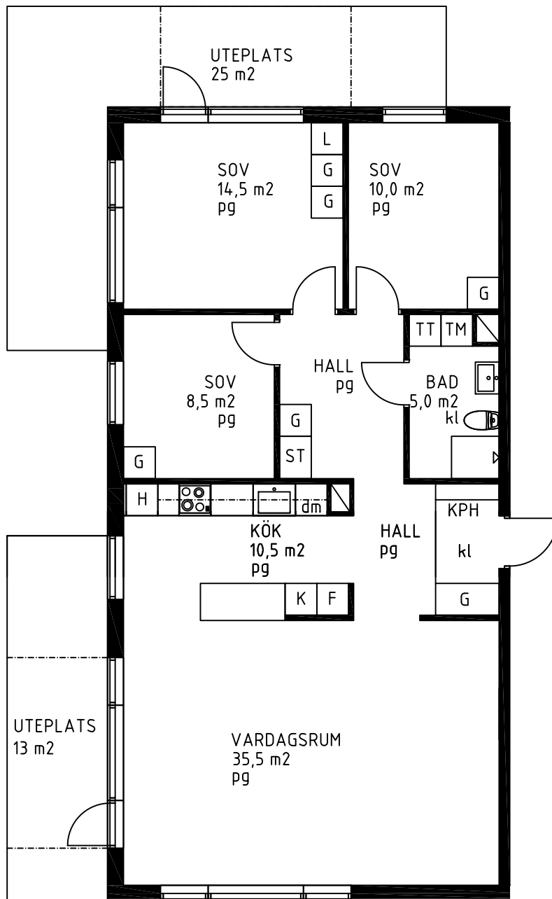
PLAN 1
